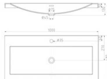
Colossum 01 - 1000 Mineral cast wash basin W1000 x H130 x D480 mm
