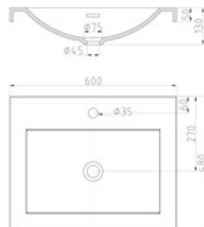
Colossum 01 - 600 Mineral cast wash basin W600 x H130 x D480 mm
