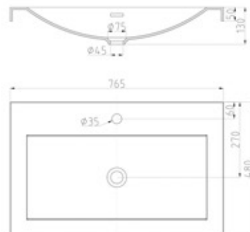
Colossum 01 - 765 Mineral cast wash basin W765 x H130 x D480 mm
